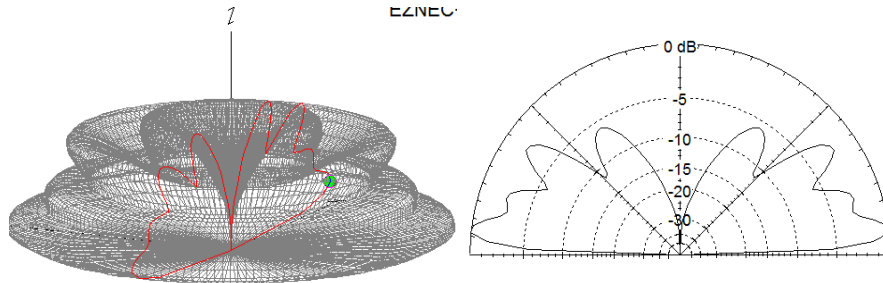
3D View
