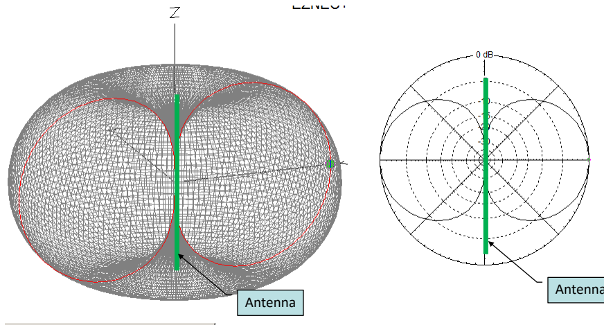
3 D view
