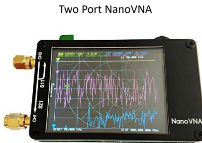
Two Port NanoVNA
