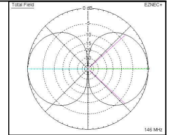
Vertical Dipole Side View
